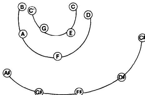
FIG. 2. The two-dimensional multidimensional scaling solution of the similarity data.
